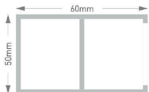
BAFFLE TUBE
